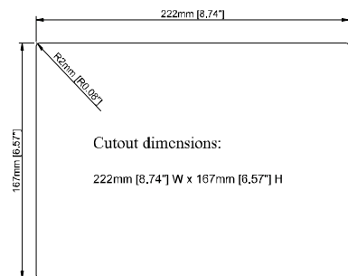
Panel Cutout
