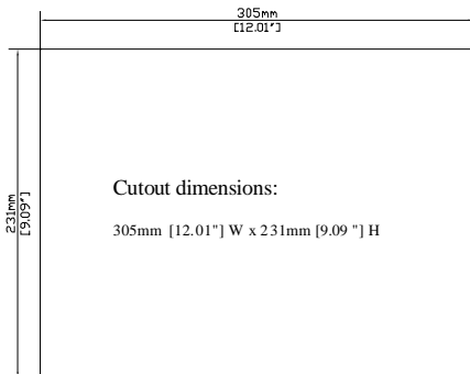
Panel Cutout
